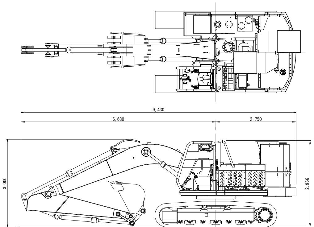
輸送姿勢 FIGURE OF TRANSPORTATION
